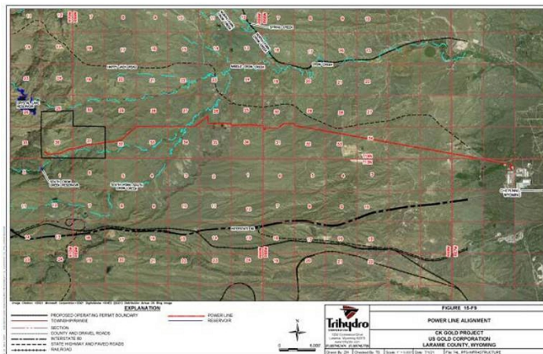
Figure 15-9 Proposed Powerline Alignment
