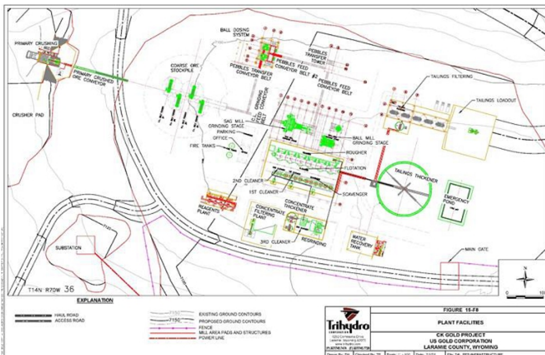
Figure 15-8 Concentrator Plan View
