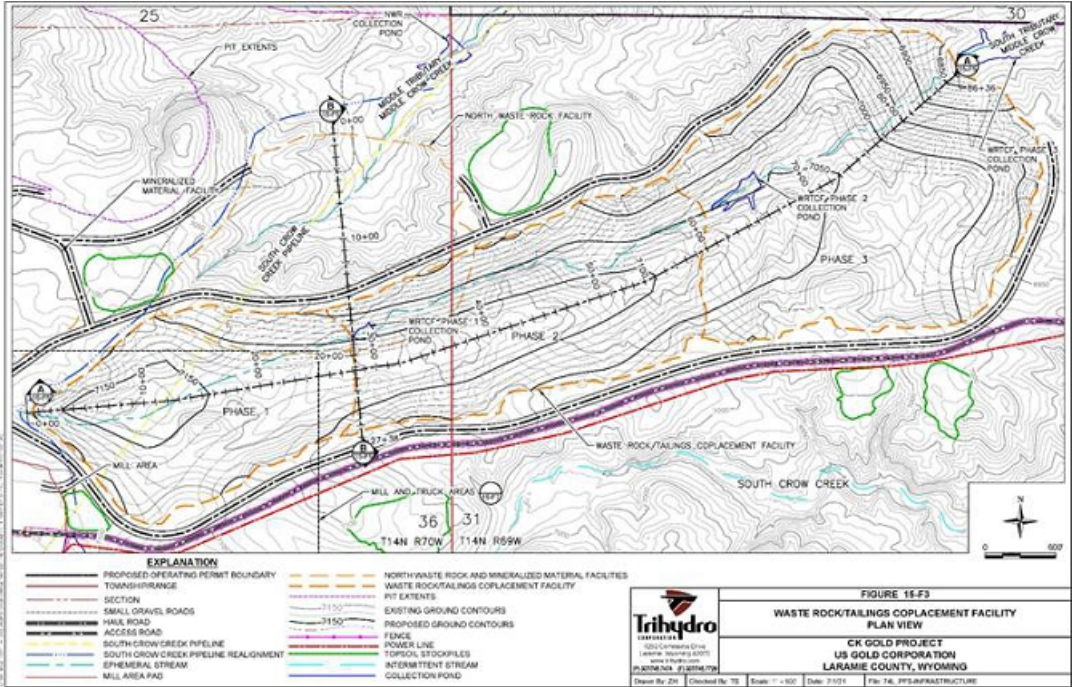
Figure 15-3 WRTCF Plan View
