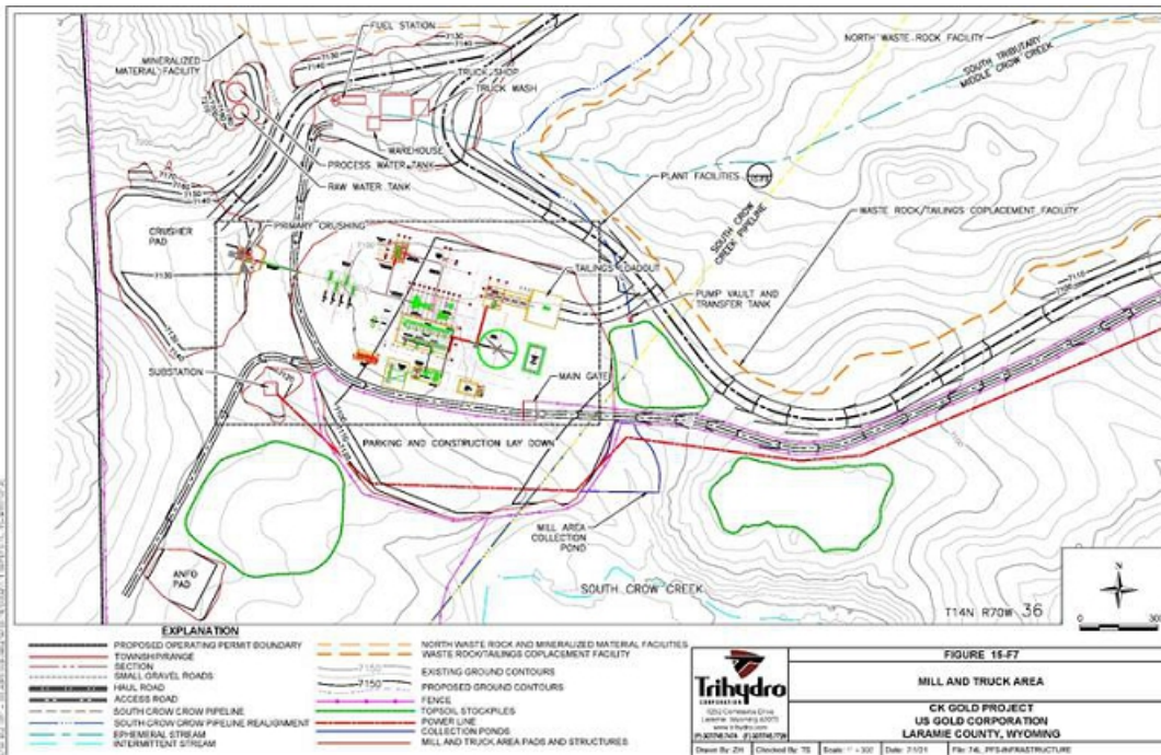
Figure 15-7 Mill and Truck Area
