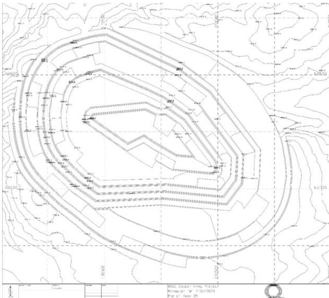
Figure 13-11 Mine Map End of Year 5
