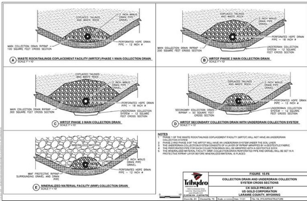
Figure 15-6 Drain System Cross Section
