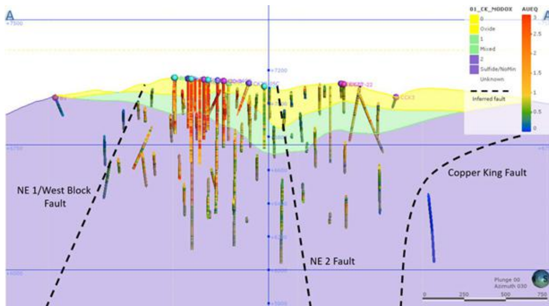
Figure 11-4 Vertical Section A-A' Looking 030° Showing Location of Interpreted NE 2 Fault Zone, Oxidation Boundaries and Drillhole Grades (AUEQ g/t)
