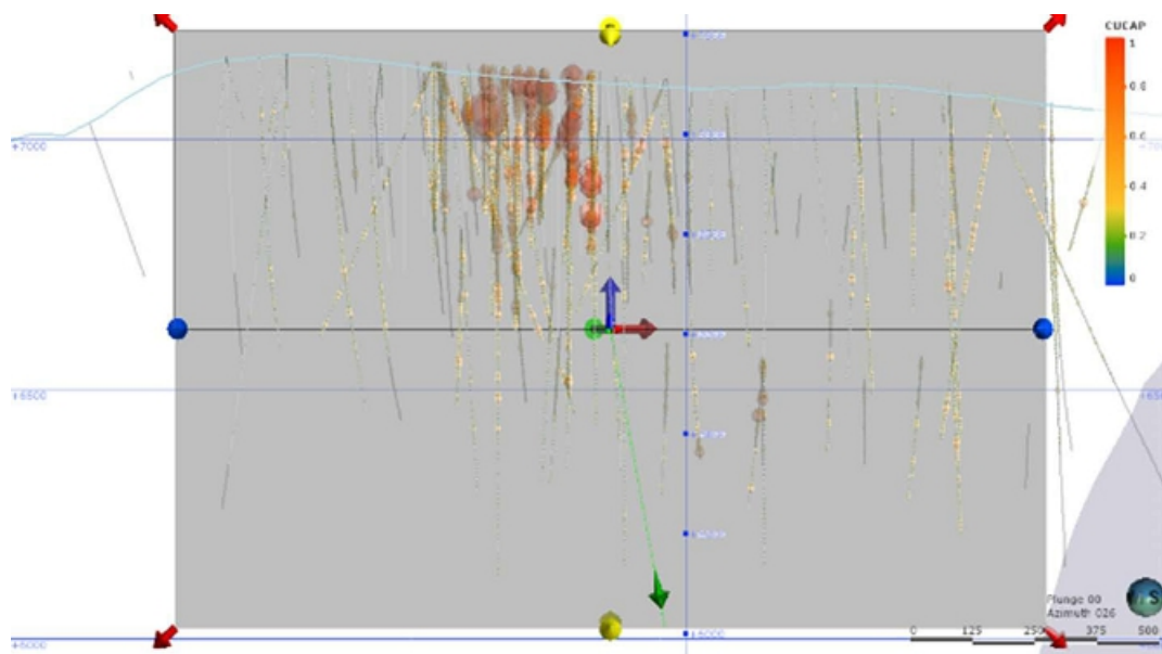
Figure 11-13 Cu Composite Points for Resource Drillholes, looking 026° at Plane of Best-fit Mineralization (green arrow indicating 100° pitch) used for Spatial Modeling (Variography)
