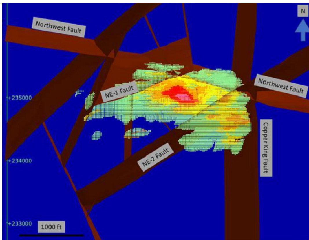
Figure 6-2 Fault Map, Blocks indicate mineralization low metal values (green) to high values (magenta)
