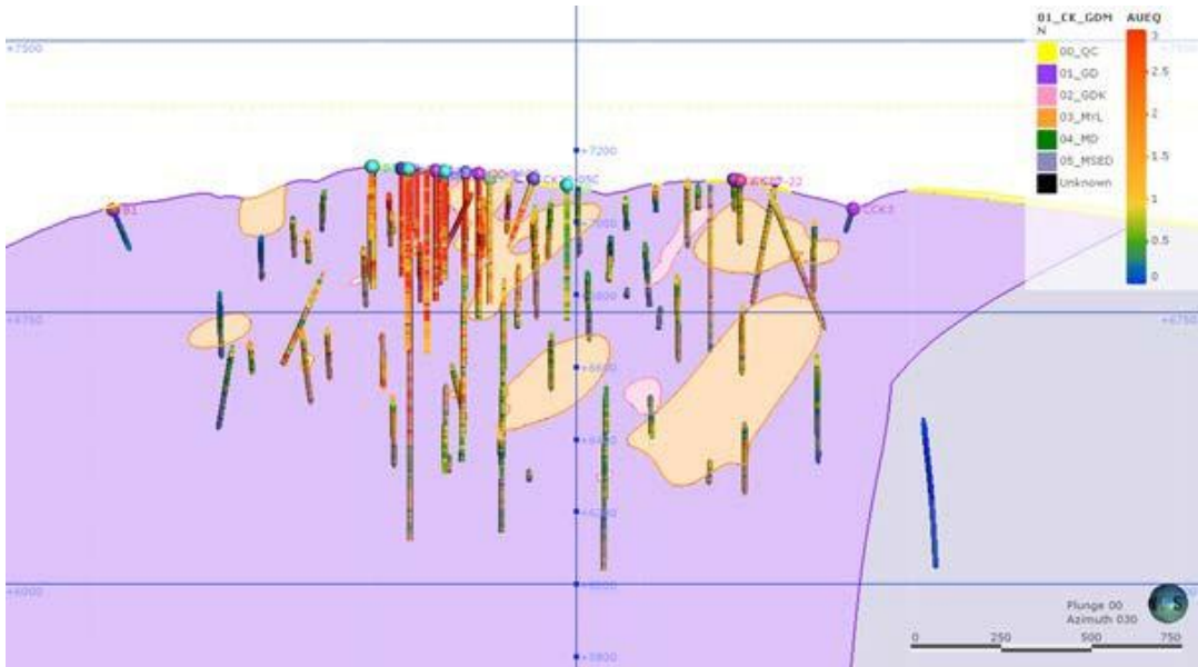
Figure 11-1 Vertical Section Looking 030deg Showing Lithologic Boundaries and Drillhole Grades (AUEQ g/t)
