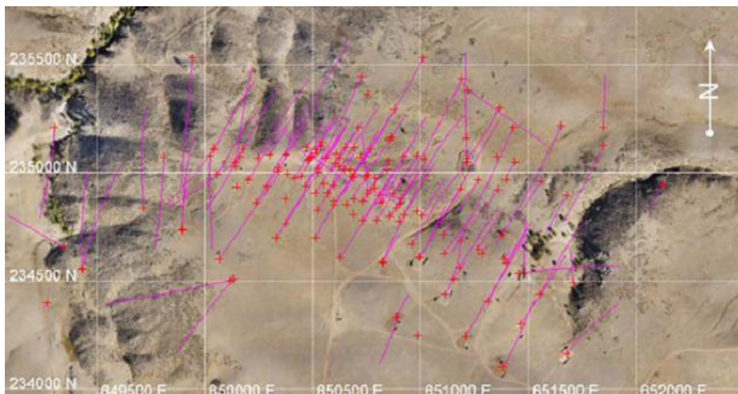
Figure 7-1 Drill hole Map
