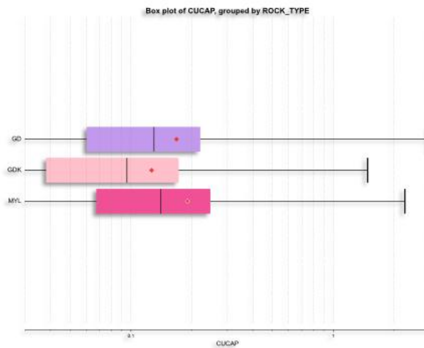
Figure 11-7 Box Plot for Cu%, Variable of the Host Rock
