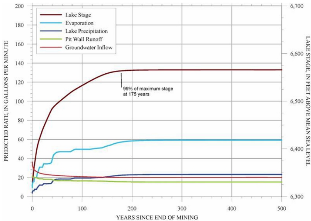
Figure 13-8 Predicted Pit Lake Water Balance
