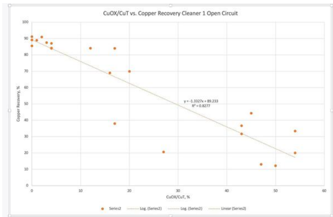
Figure 10-3 Variability Samples, Copper Recovery v CuOx/CuT
