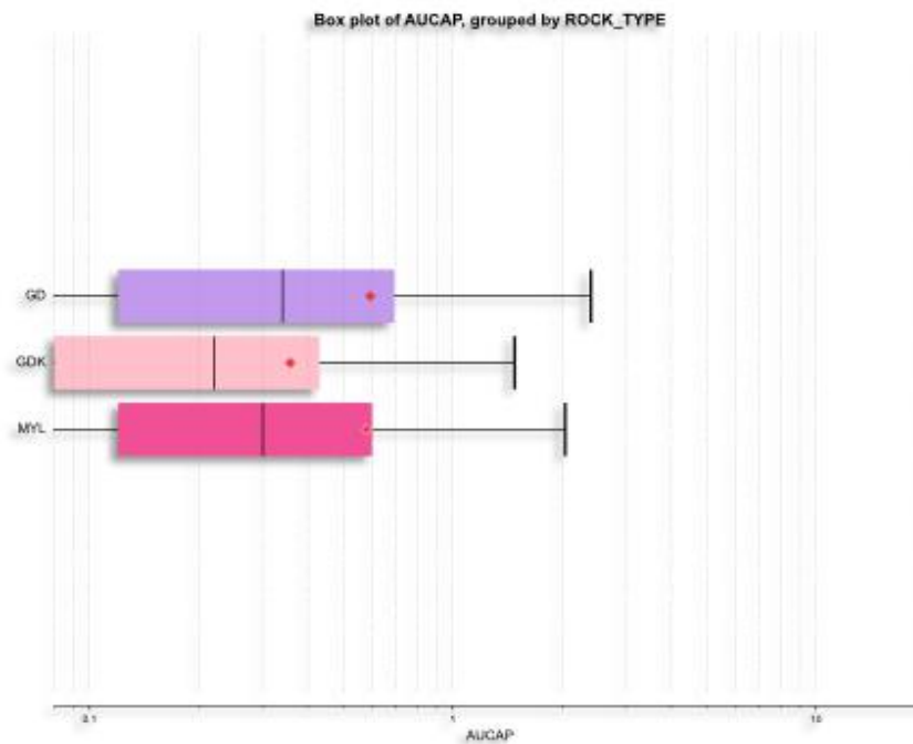
Figure 11-6 Box Plot for Au g/t, Variable of Host Rock
