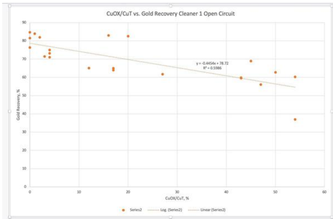
Figure 10-2 Variability Samples, Au Recovery v CuOx/CuT
