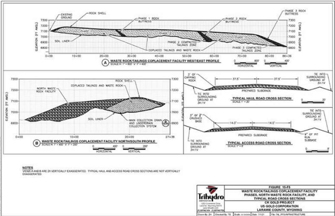
Figure 15-5 Facility Cross Sections
