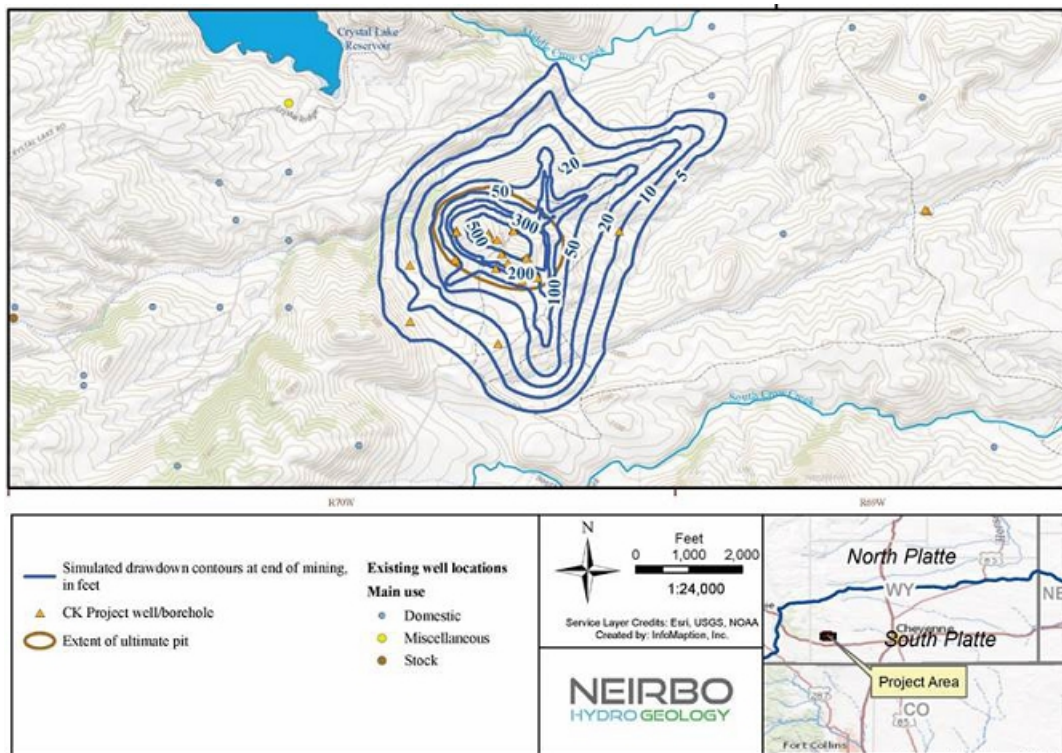
Figure 13-5 Predicted Groundwater Drawdown at End of Mining
