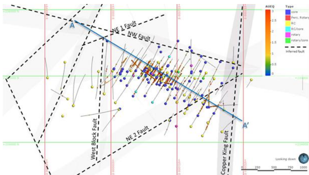
Figure 11-3 Fault Map with Drillhole Grades ( \geq 1.5 g/t AUEQ)
