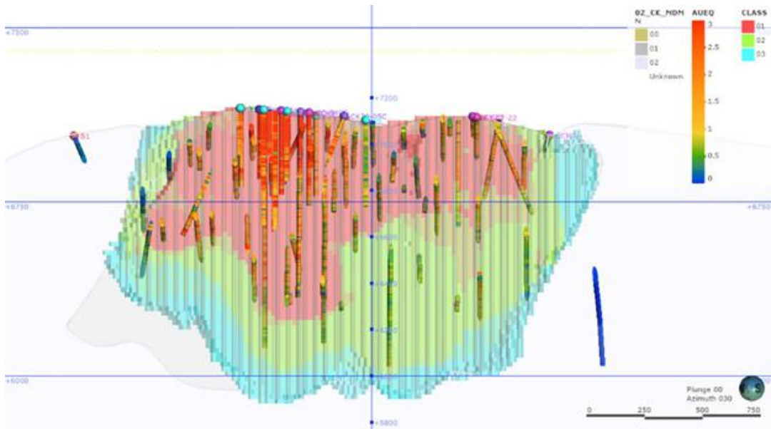
Figure 11-15 Longitudinal (100 ft field of view), looking 030° through the 3D block model, showing Measured (red), Indicated (green) and Inferred (blue) class resources with a \geq 0.3 g/t AUEQ cutoff applied.
