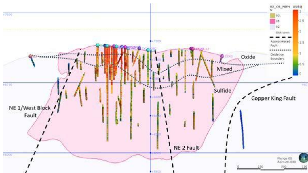
Figure 11-5 Vertical Section Looking 030° Showing Mineralized Domain, Modeled Oxidation, Structures and Drillhole Grades (AUEQ g/t)
