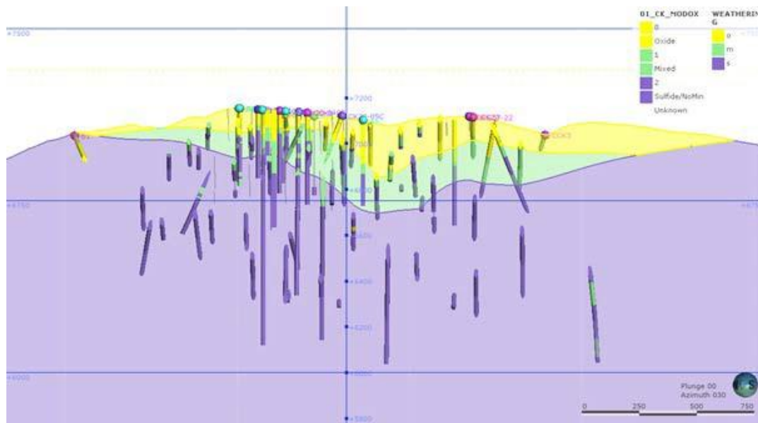
Figure 11-2 Vertical Section Looking 030° Showing Oxidation Boundaries and Drillhole Weathering
