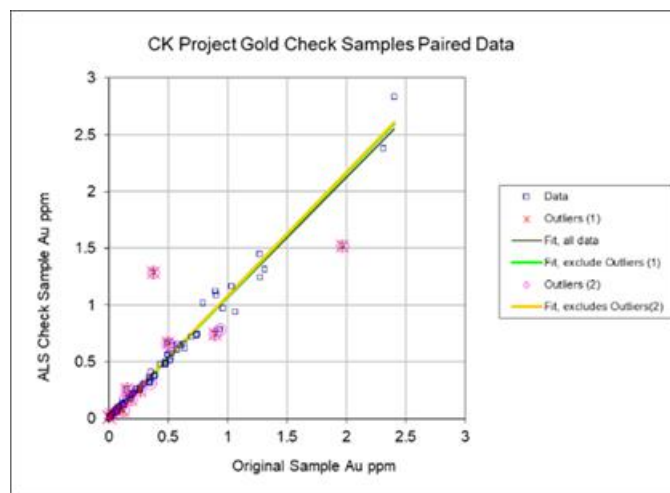
Figure 8-1 Umpire Analysis Au Correlation
