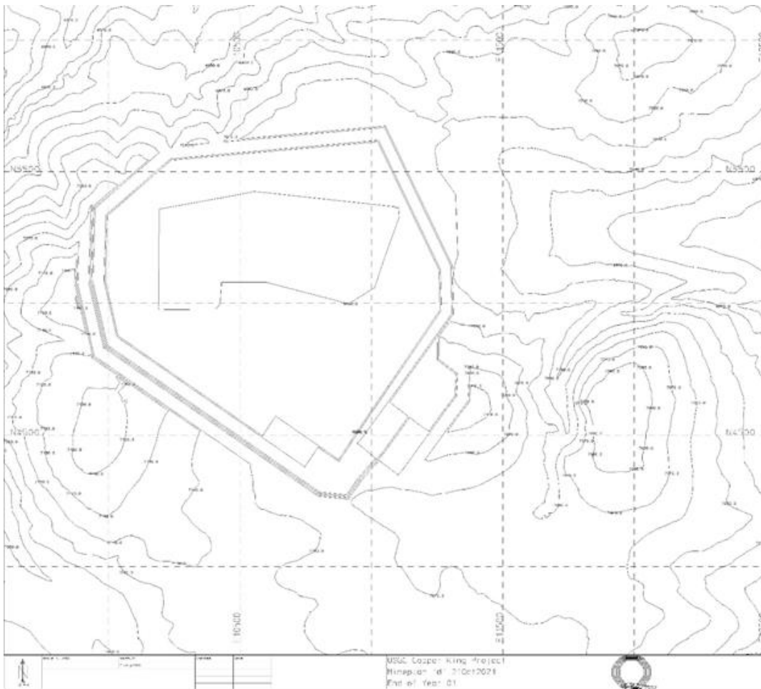
Figure 13-9 Mine Map End of Year 1
