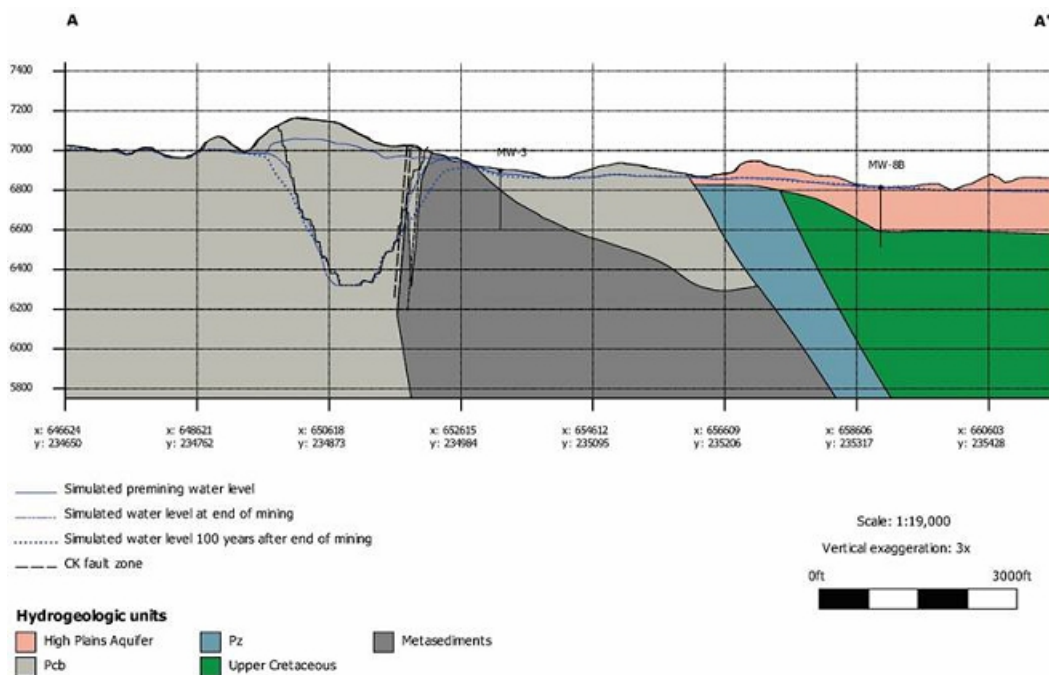
Figure 13-7 Section A-A' showing predicted drawdown at the end of mining and 100 years after mining ends.
