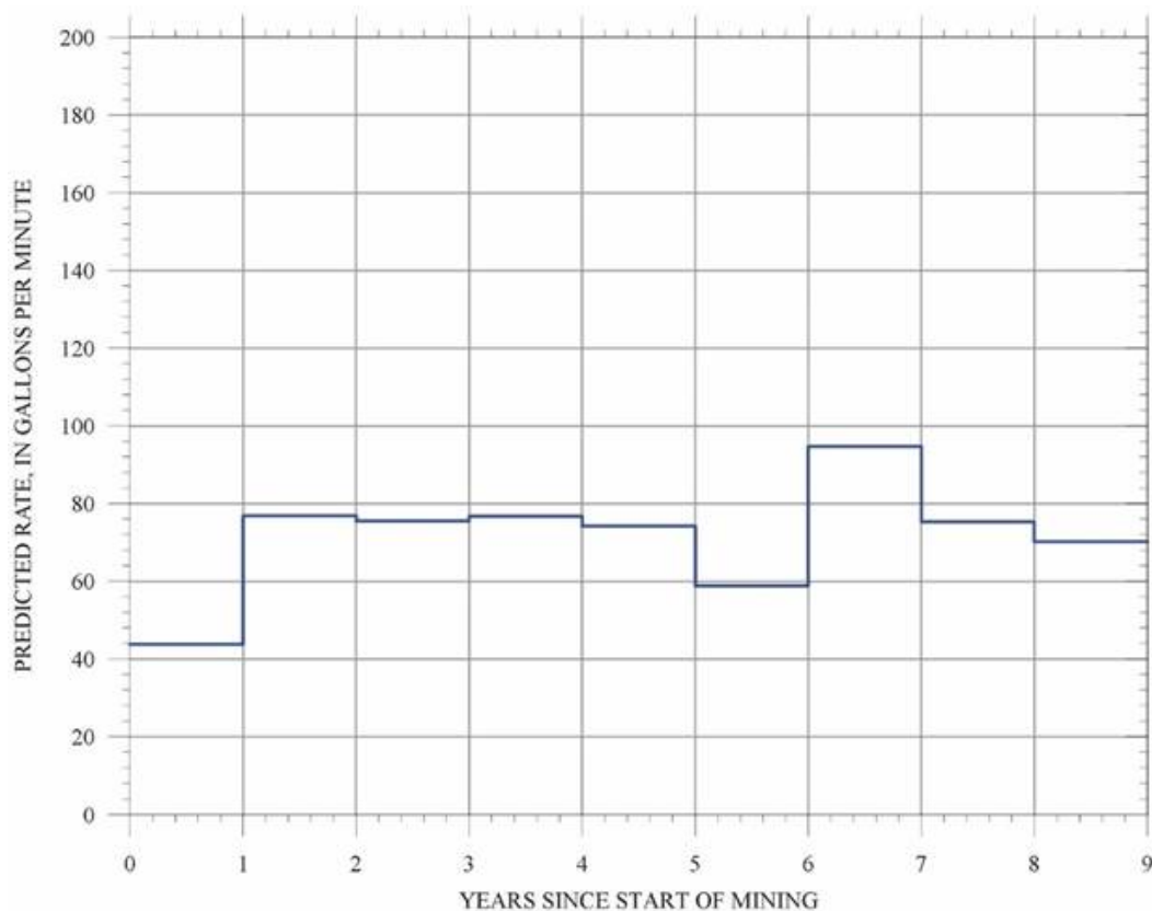
Figure 13-4 Predicted Open Pit Inflows
