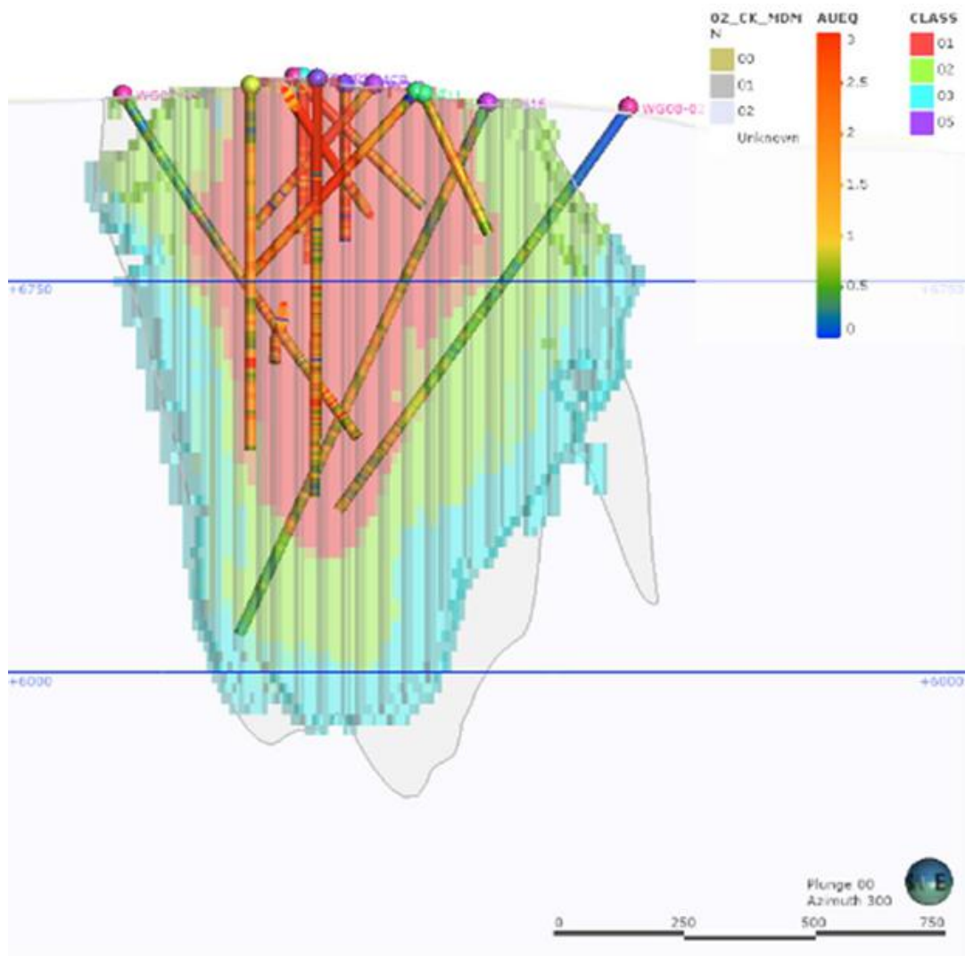
Figure 11-16 Cross-section slice (100 ft field of view), looking 300° through the 3D block model, showing Measured (red), Indicated (green) and Inferred (blue) class resources with a \geq 0.3 g/t AUEQ cutoff applied.
