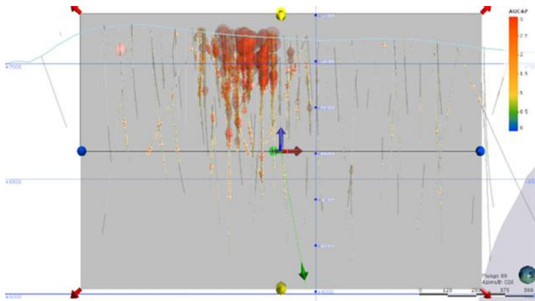
Figure 11-12 Au Composite Points for Resource Drillholes, looking 026° at Plane of Best-fit Mineralization (green arrow indicating 100° pitch) used for Spatial Modeling (Variography)
